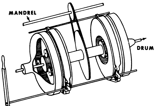
Figure 8-8. Chain-driven feed works with lever-controlled brake bevels on split housing.
